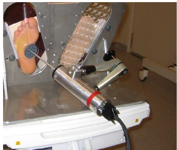
Fig. 1. Vibration probe attached to the subject's arch of the foot with a contact force of 0.05 N to the skin surface. The contact area of the skin surface and the indenter was circular and about 20 cm 2 . The Moving Magnet Actuator System was regulated, so that the contact force was kept constant at 0.05 N throughout the fMRI measurement.
